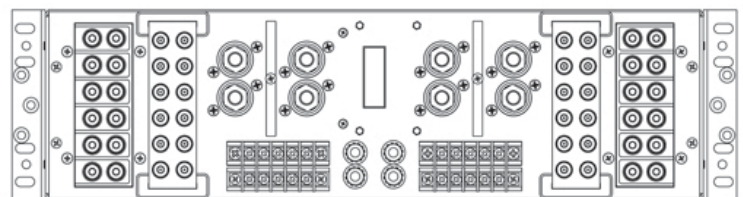
Fig. 2: 350CB06 Rear View Drawing
